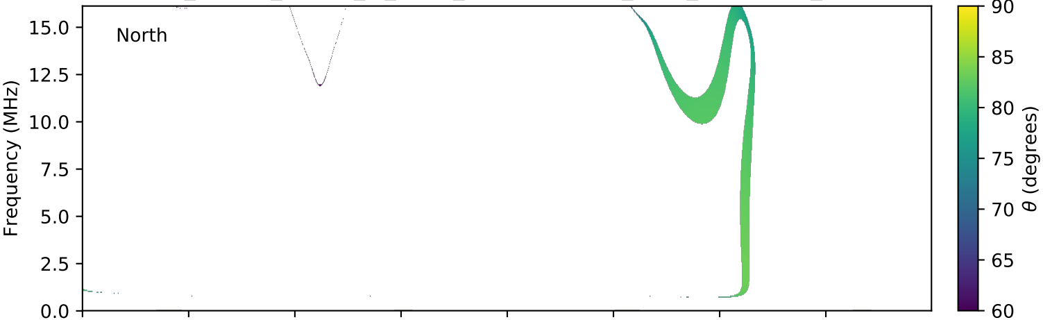
expres_cassini_jupiter_io_isaac_lossc-wid1deg_3kev_20000627_v01.cdf
