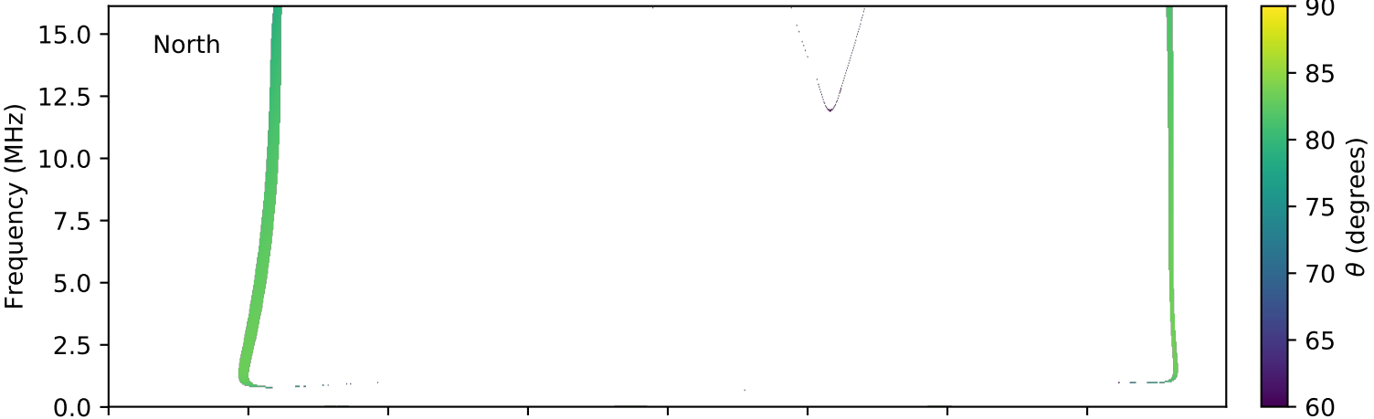
expres_cassini_jupiter_io_isaac_lossc-wid1deg_3kev_20000618_v01.cdf
