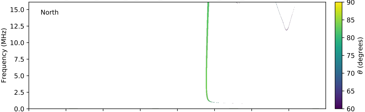
expres_cassini_jupiter_io_isaac_lossc-wid1deg_3kev_20000614_v01.cdf
