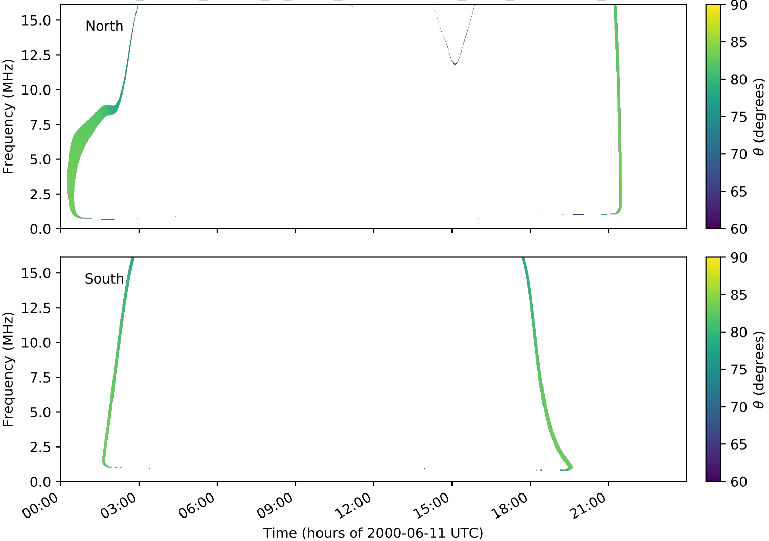
expres_cassini_jupiter_io_isaac_lossc-wid1deg_3kev_20000611_v01.cdf
