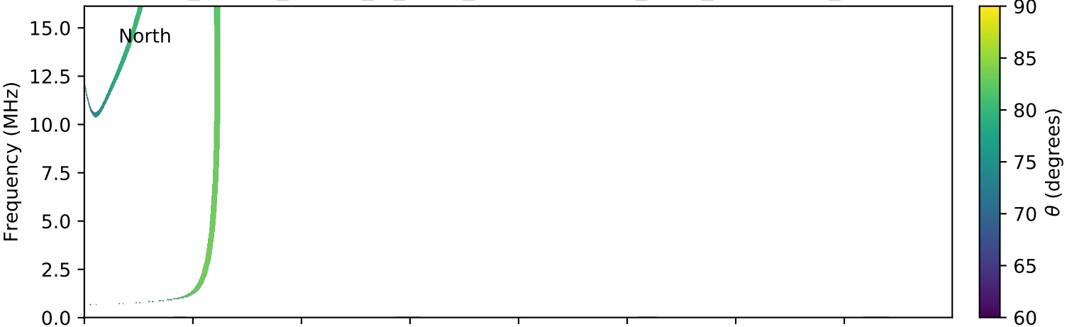
expres_cassini_jupiter_io_isaac_lossc-wid1deg_3kev_20000610_v01.cdf
