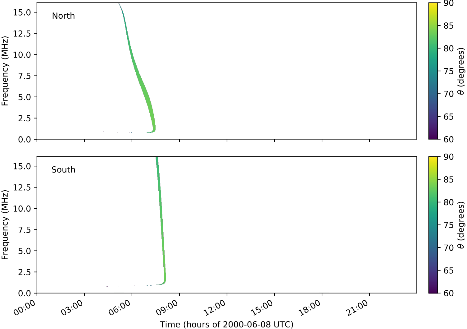
expres_cassini_jupiter_io_isaac_lossc-wid1deg_3kev_20000608_v01.cdf
