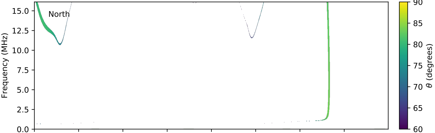
expres_cassini_jupiter_io_isaac_lossc-wid1deg_3kev_20000604_v01.cdf
