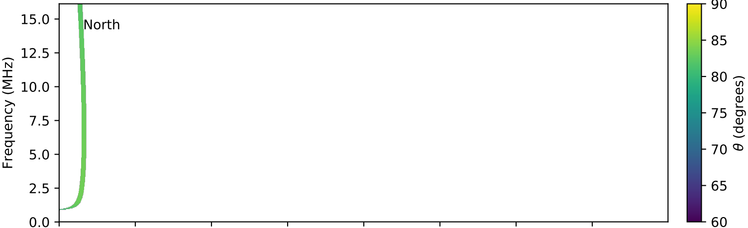
expres_cassini_jupiter_ganymede_isaac_lossc-wid1deg_3kev_20000630_v01.cdf
