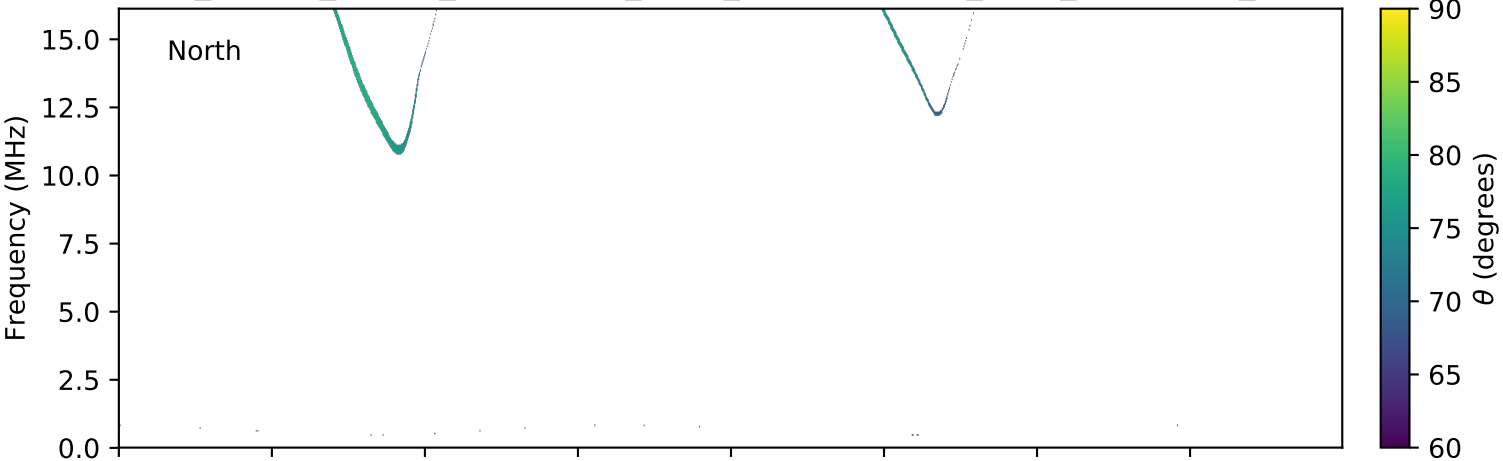
expres_cassini_jupiter_ganymede_isaac_lossc-wid1deg_3kev_20000627_v01.cdf
