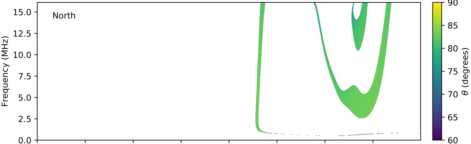
expres_cassini_jupiter_ganymede_isaac_lossc-wid1deg_3kev_20000626_v01.cdf
