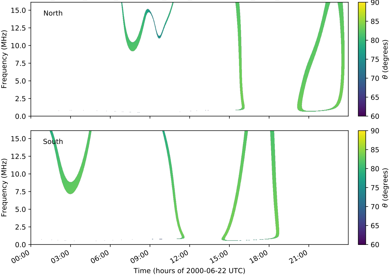
expres_cassini_jupiter_ganymede_isaac_lossc-wid1deg_3kev_20000622_v01.cdf
