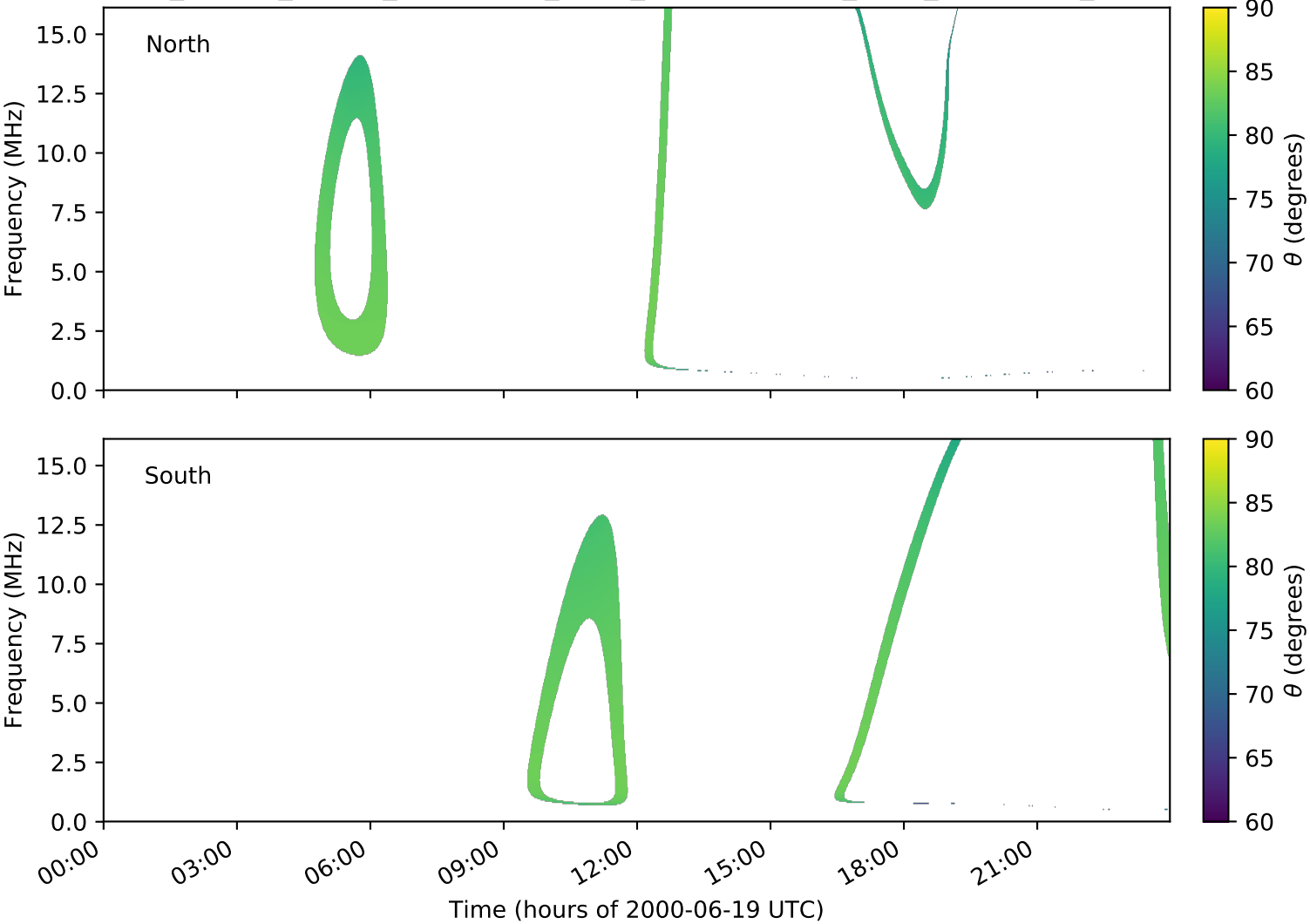
expres_cassini_jupiter_ganymede_isaac_lossc-wid1deg_3kev_20000619_v01.cdf
