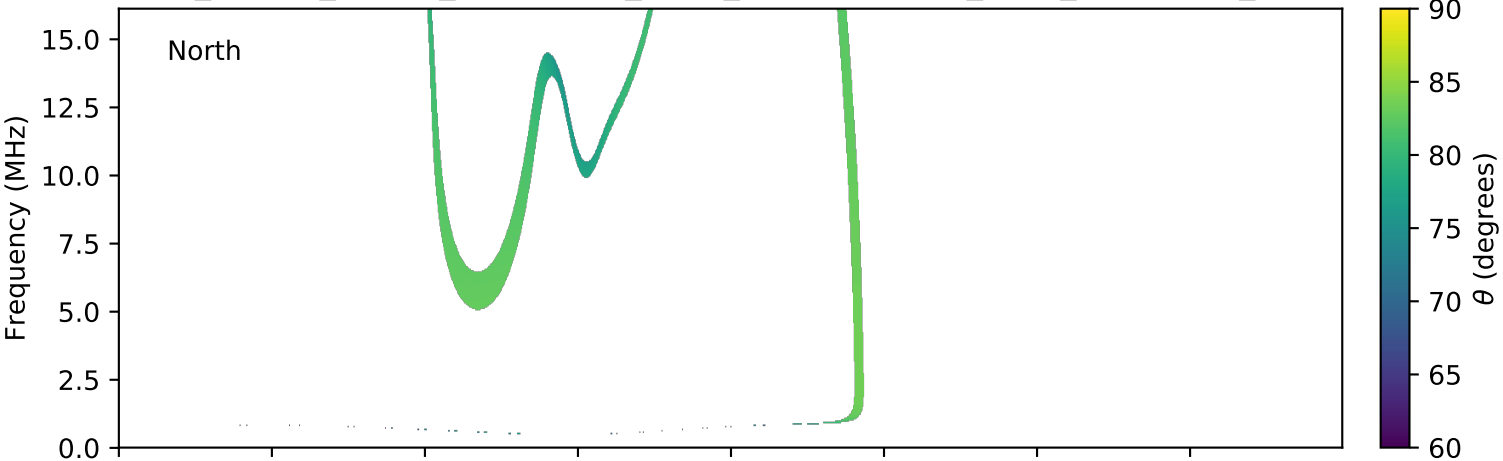
expres_cassini_jupiter_ganymede_isaac_lossc-wid1deg_3kev_20000615_v01.cdf
