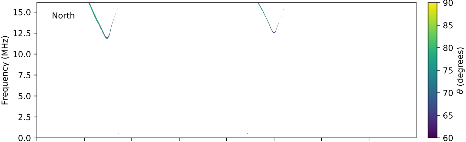
expres_cassini_jupiter_ganymede_isaac_lossc-wid1deg_3kev_20000613_v01.cdf
