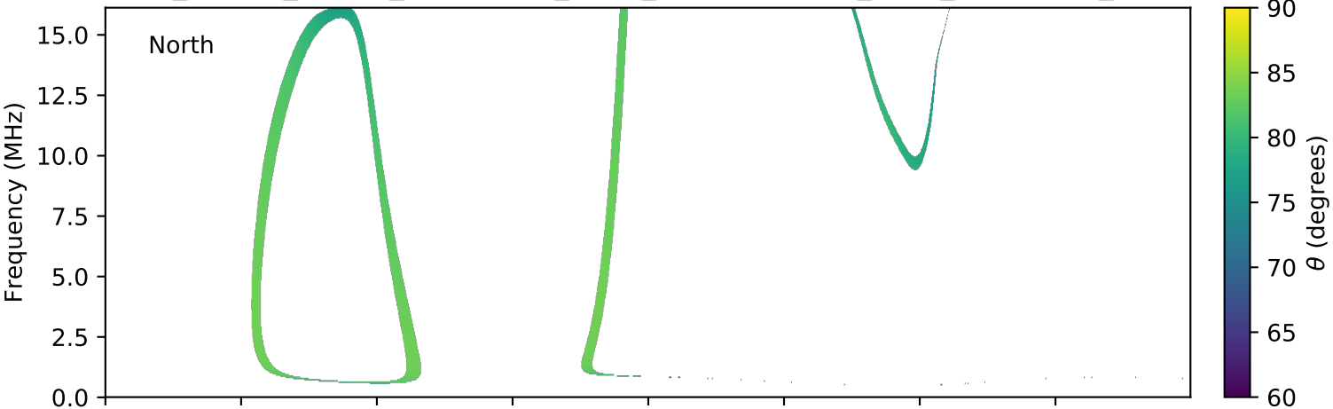
expres_cassini_jupiter_ganymede_isaac_lossc-wid1deg_3kev_20000612_v01.cdf
