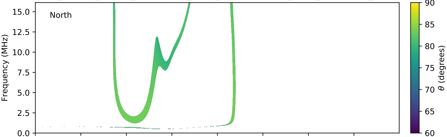
expres_cassini_jupiter_ganymede_isaac_lossc-wid1deg_3kev_20000608_v01.cdf
