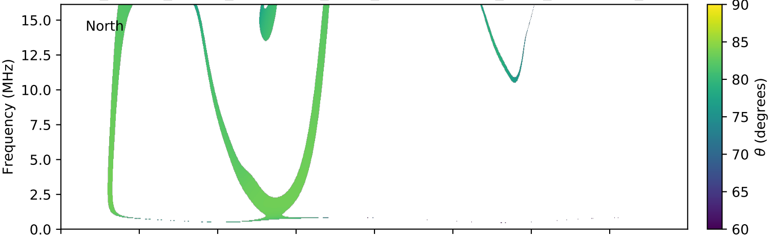
expres_cassini_jupiter_ganymede_isaac_lossc-wid1deg_3kev_20000605_v01.cdf
