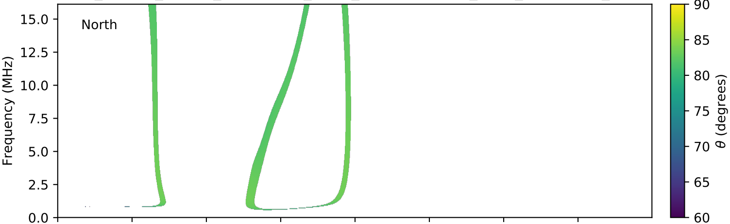
expres_cassini_jupiter_ganymede_isaac_lossc-wid1deg_3kev_20000601_v01.cdf
