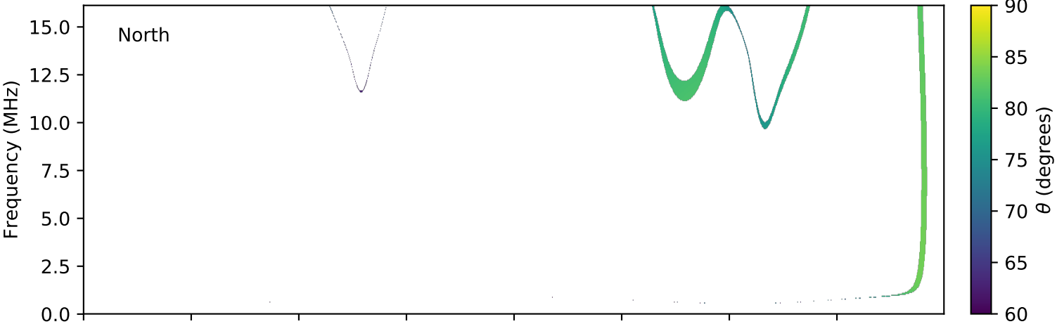
expres_cassini_jupiter_europa_isaac_lossc-wid1deg_3kev_20000627_v01.cdf
