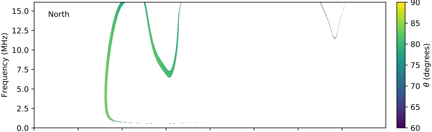
expres_cassini_jupiter_europa_isaac_lossc-wid1deg_3kev_20000626_v01.cdf
