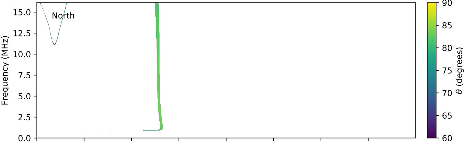
expres_cassini_jupiter_europa_isaac_lossc-wid1deg_3kev_20000624_v01.cdf
