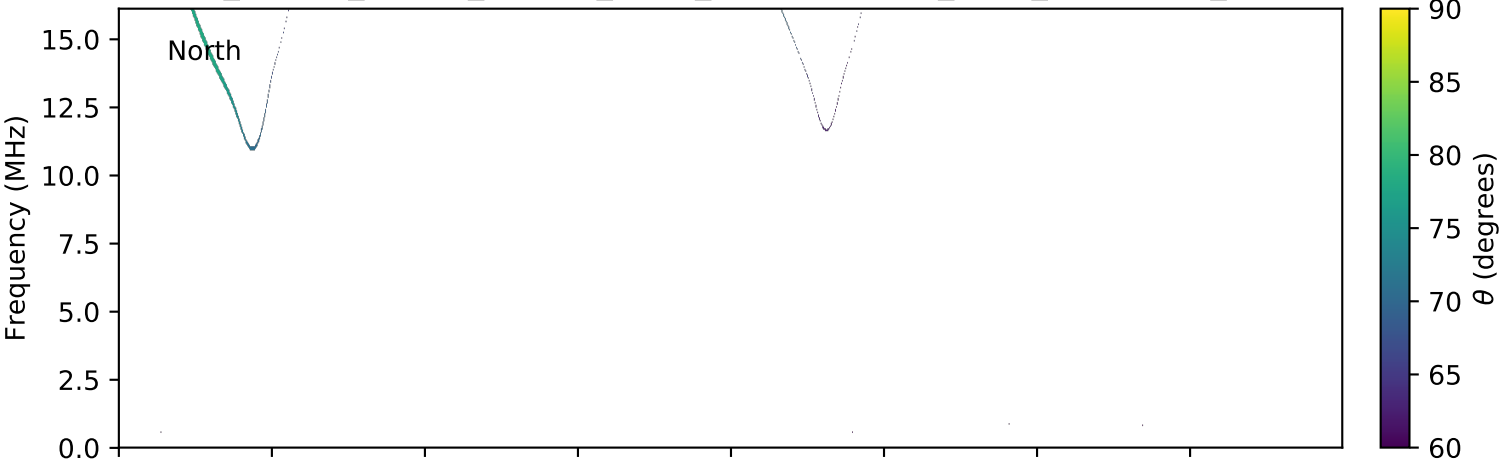
expres_cassini_jupiter_europa_isaac_lossc-wid1deg_3kev_20000623_v01.cdf
