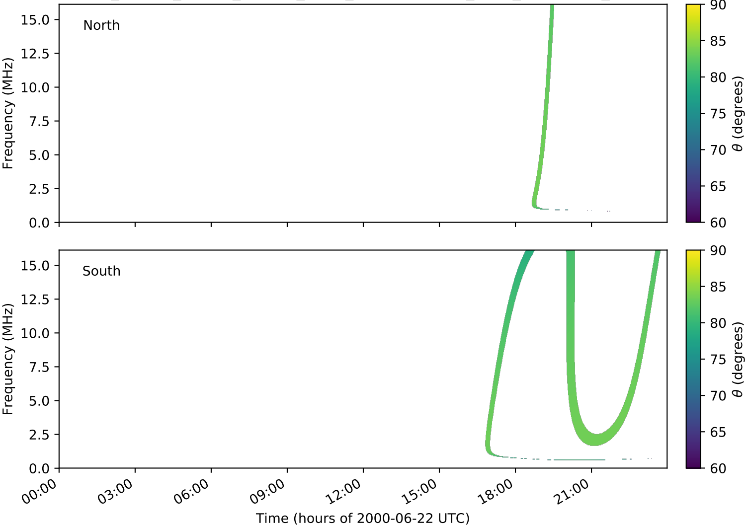
expres_cassini_jupiter_europa_isaac_lossc-wid1deg_3kev_20000622_v01.cdf
