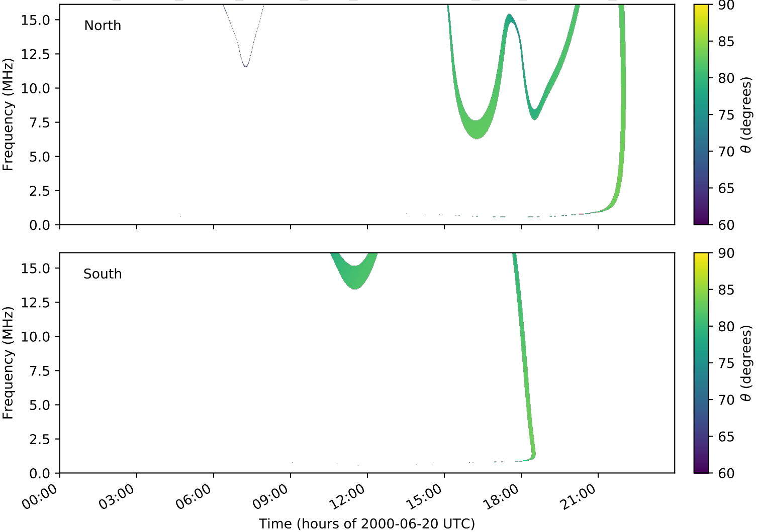
expres_cassini_jupiter_europa_isaac_lossc-wid1deg_3kev_20000620_v01.cdf
