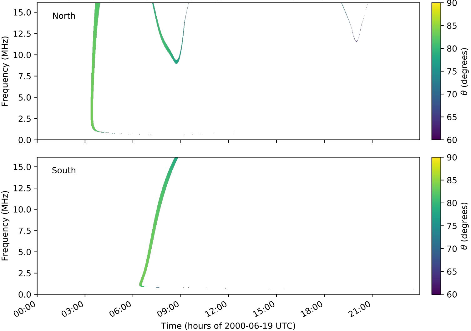
expres_cassini_jupiter_europa_isaac_lossc-wid1deg_3kev_20000619_v01.cdf
