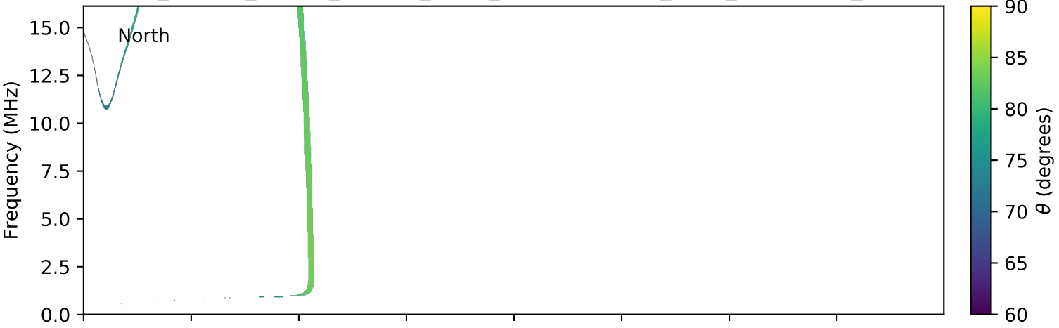
expres_cassini_jupiter_europa_isaac_lossc-wid1deg_3kev_20000617_v01.cdf
