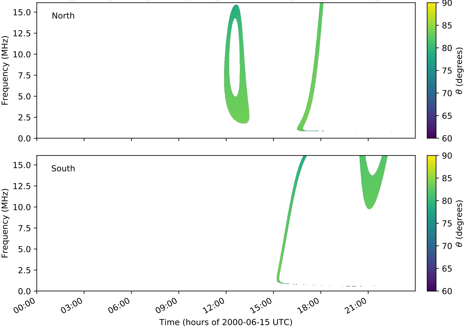
expres_cassini_jupiter_europa_isaac_lossc-wid1deg_3kev_20000615_v01.cdf
