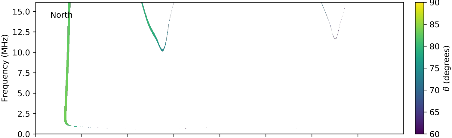
expres_cassini_jupiter_europa_isaac_lossc-wid1deg_3kev_20000612_v01.cdf
