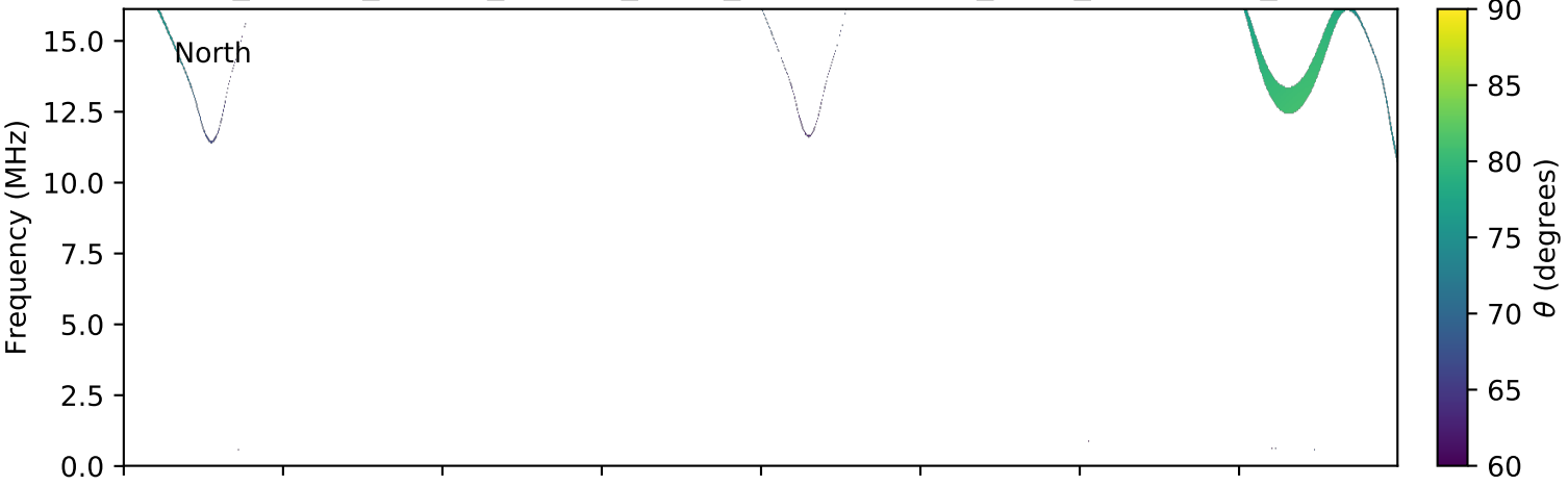
expres_cassini_jupiter_europa_isaac_lossc-wid1deg_3kev_20000609_v01.cdf
