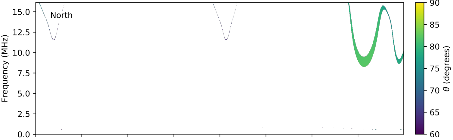
expres_cassini_jupiter_europa_isaac_lossc-wid1deg_3kev_20000602_v01.cdf
