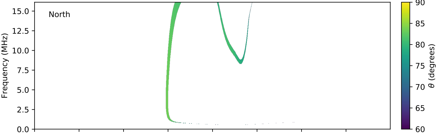
expres_cassini_jupiter_europa_isaac_lossc-wid1deg_3kev_20000601_v01.cdf
