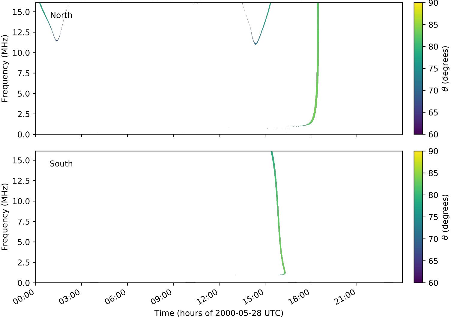
expres_cassini_jupiter_io_isaac_lossc-wid1deg_3kev_20000528_v01.cdf
