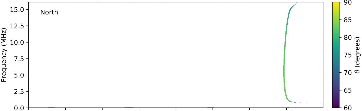
expres_cassini_jupiter_io_isaac_lossc-wid1deg_3kev_20000527_v01.cdf
