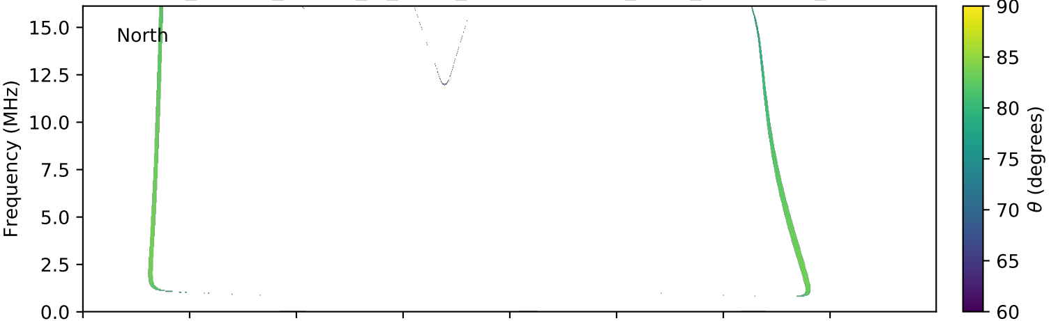
expres_cassini_jupiter_io_isaac_lossc-wid1deg_3kev_20000519_v01.cdf
