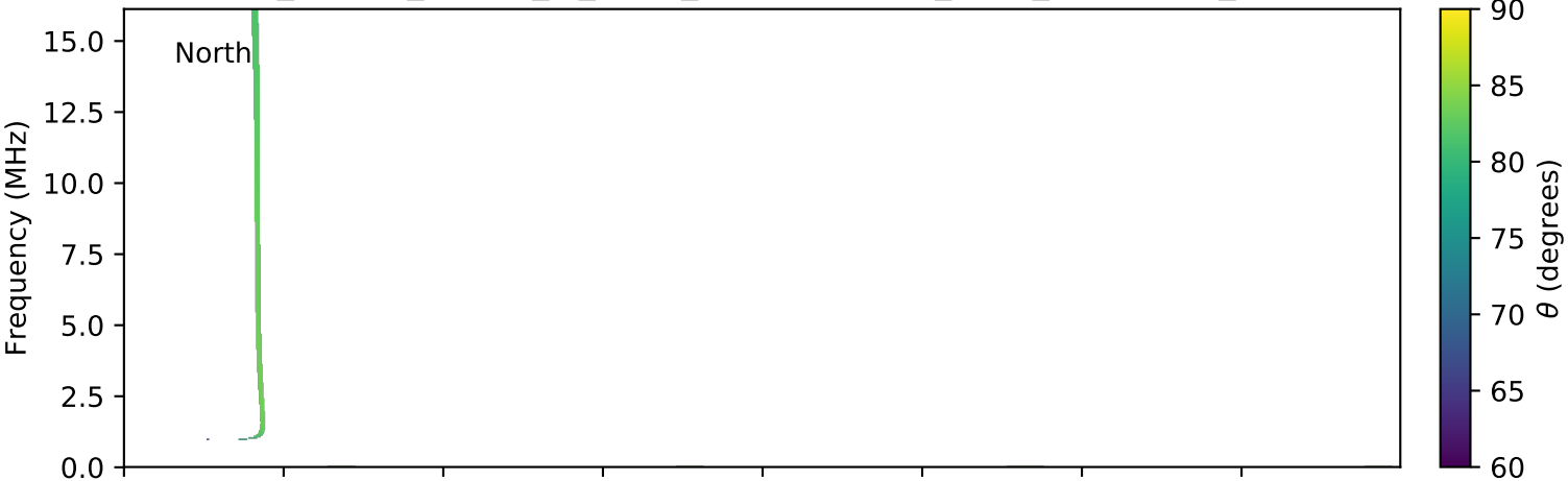
expres_cassini_jupiter_io_isaac_lossc-wid1deg_3kev_20000518_v01.cdf
