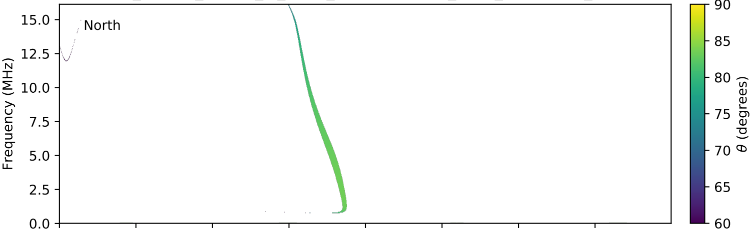
expres_cassini_jupiter_io_isaac_lossc-wid1deg_3kev_20000507_v01.cdf
