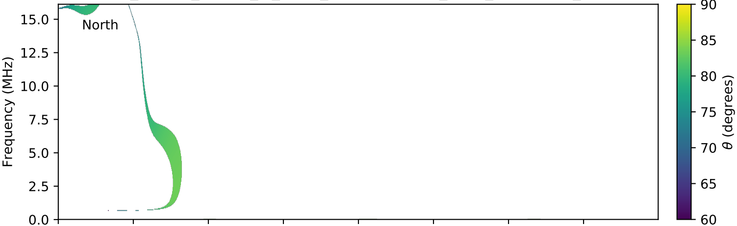
expres_cassini_jupiter_io_isaac_lossc-wid1deg_3kev_20000502_v01.cdf
