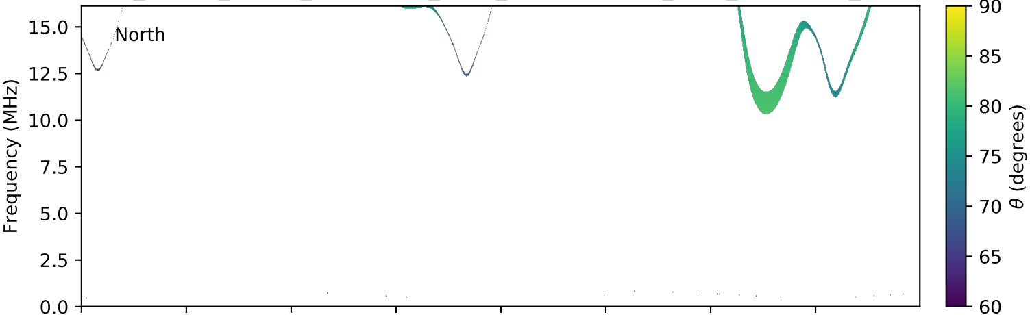
expres_cassini_jupiter_ganymede_isaac_lossc-wid1deg_3kev_20000531_v01.cdf
