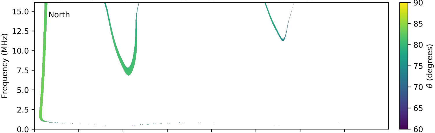
expres_cassini_jupiter_ganymede_isaac_lossc-wid1deg_3kev_20000529_v01.cdf
