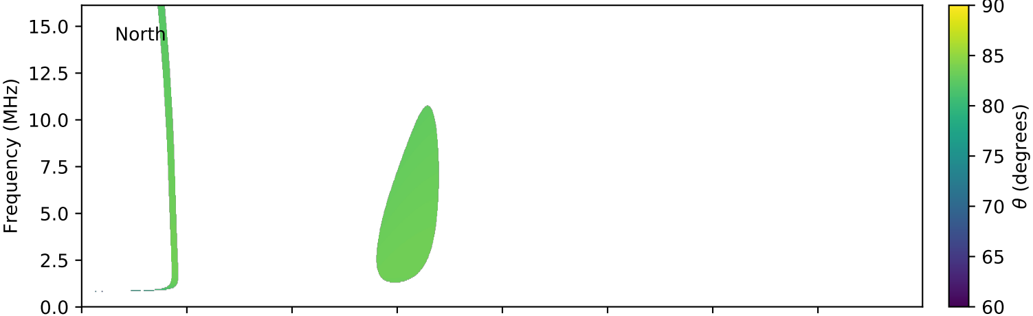
expres_cassini_jupiter_ganymede_isaac_lossc-wid1deg_3kev_20000525_v01.cdf
