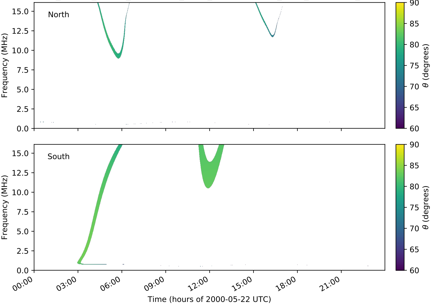
expres_cassini_jupiter_ganymede_isaac_lossc-wid1deg_3kev_20000522_v01.cdf
