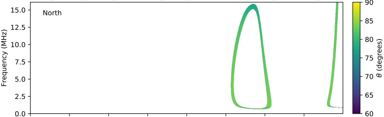
expres_cassini_jupiter_ganymede_isaac_lossc-wid1deg_3kev_20000521_v01.cdf
