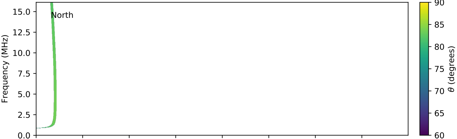
expres_cassini_jupiter_ganymede_isaac_lossc-wid1deg_3kev_20000518_v01.cdf
