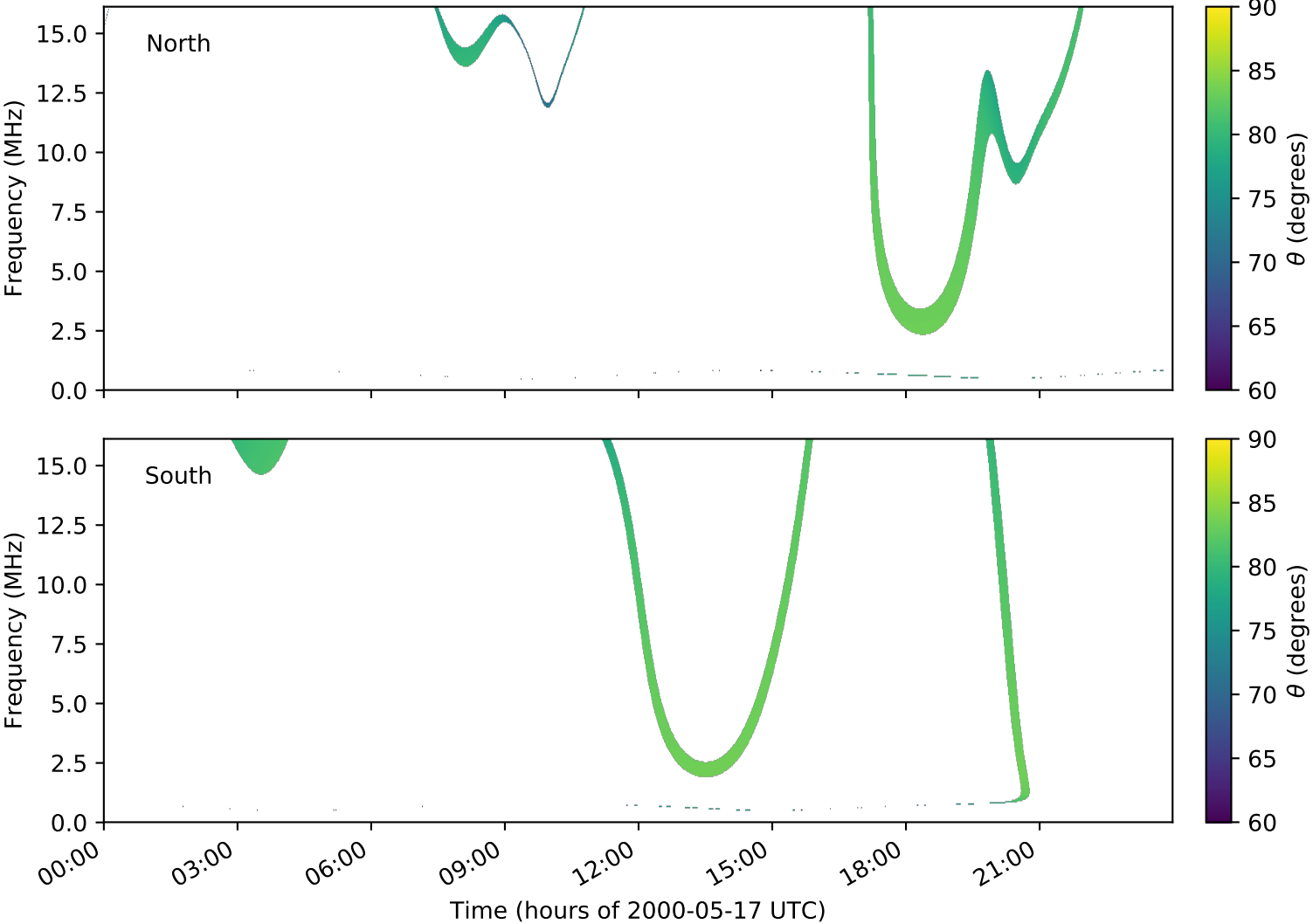
expres_cassini_jupiter_ganymede_isaac_lossc-wid1deg_3kev_20000517_v01.cdf
