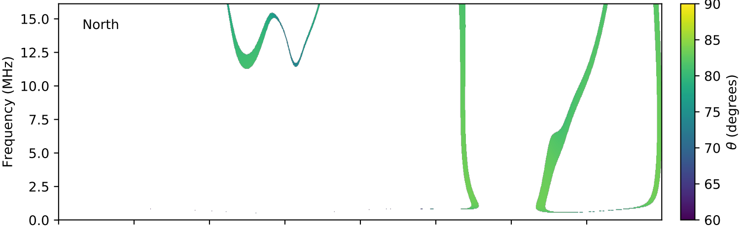
expres_cassini_jupiter_ganymede_isaac_lossc-wid1deg_3kev_20000510_v01.cdf
