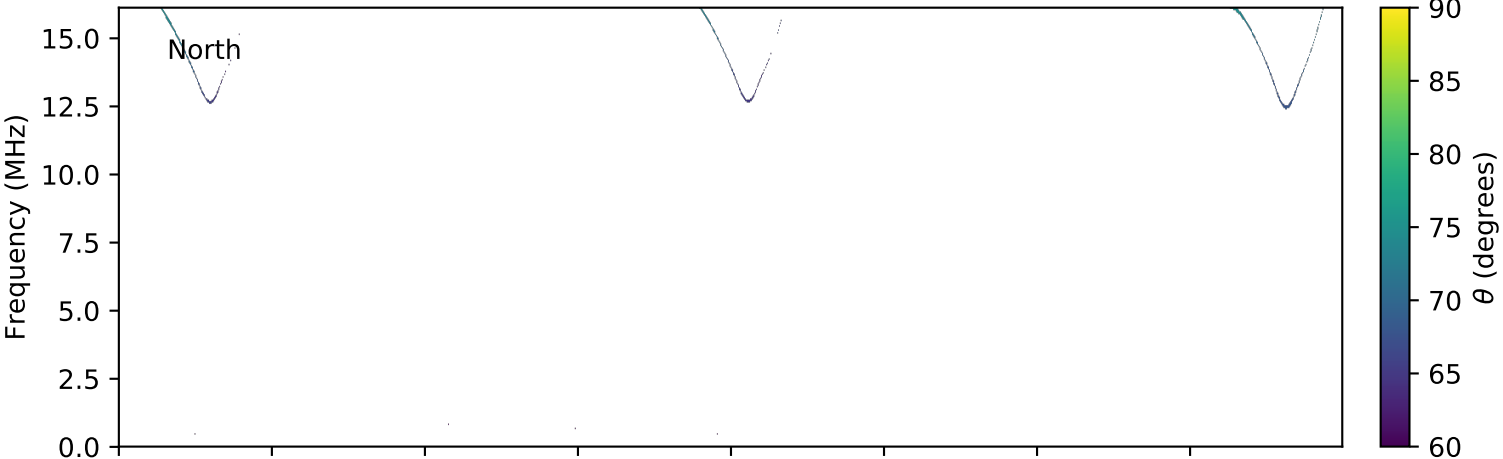
expres_cassini_jupiter_ganymede_isaac_lossc-wid1deg_3kev_20000509_v01.cdf
