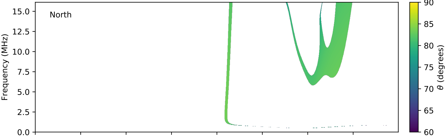
expres_cassini_jupiter_ganymede_isaac_lossc-wid1deg_3kev_20000507_v01.cdf
