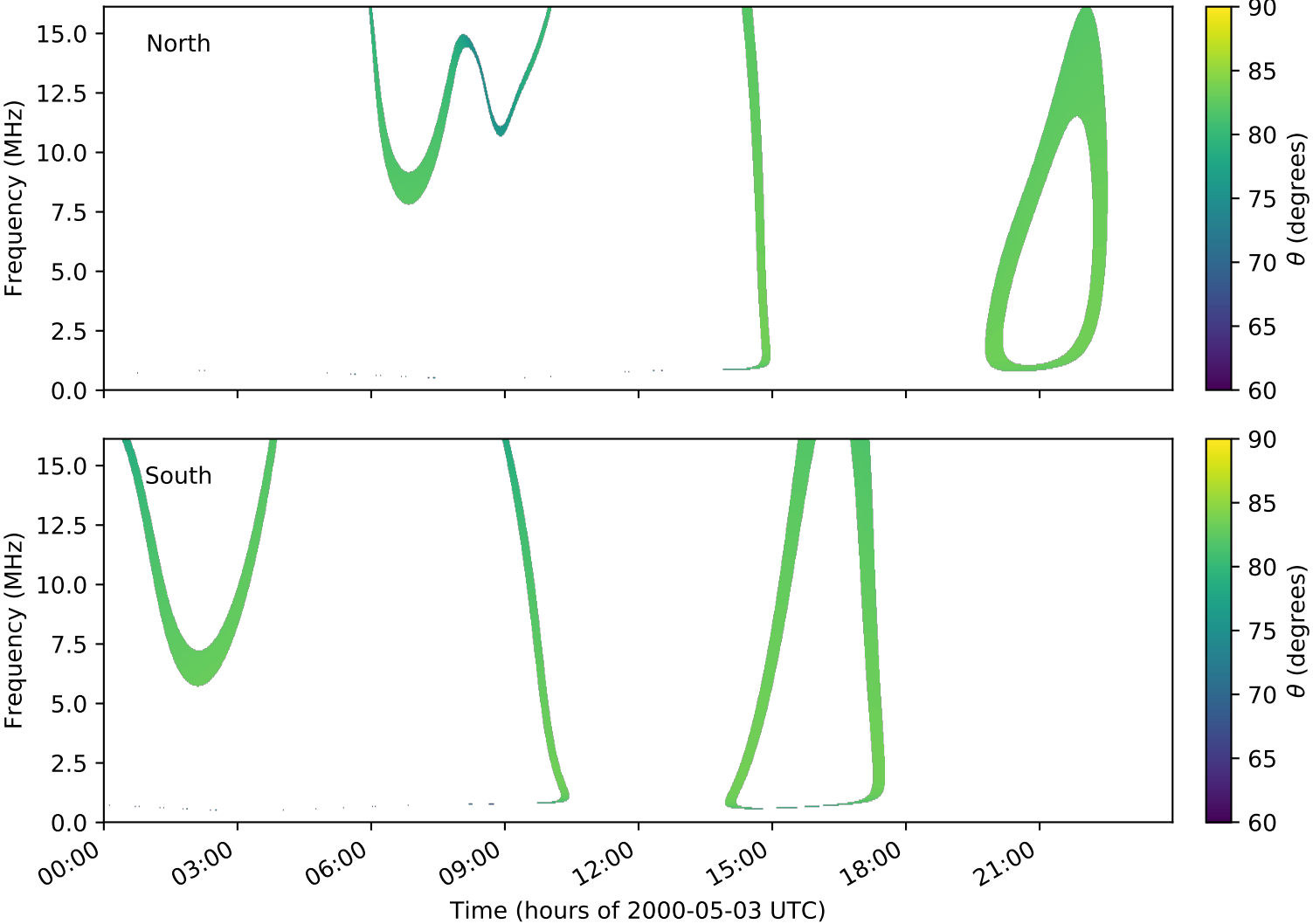
expres_cassini_jupiter_ganymede_isaac_lossc-wid1deg_3kev_20000503_v01.cdf
