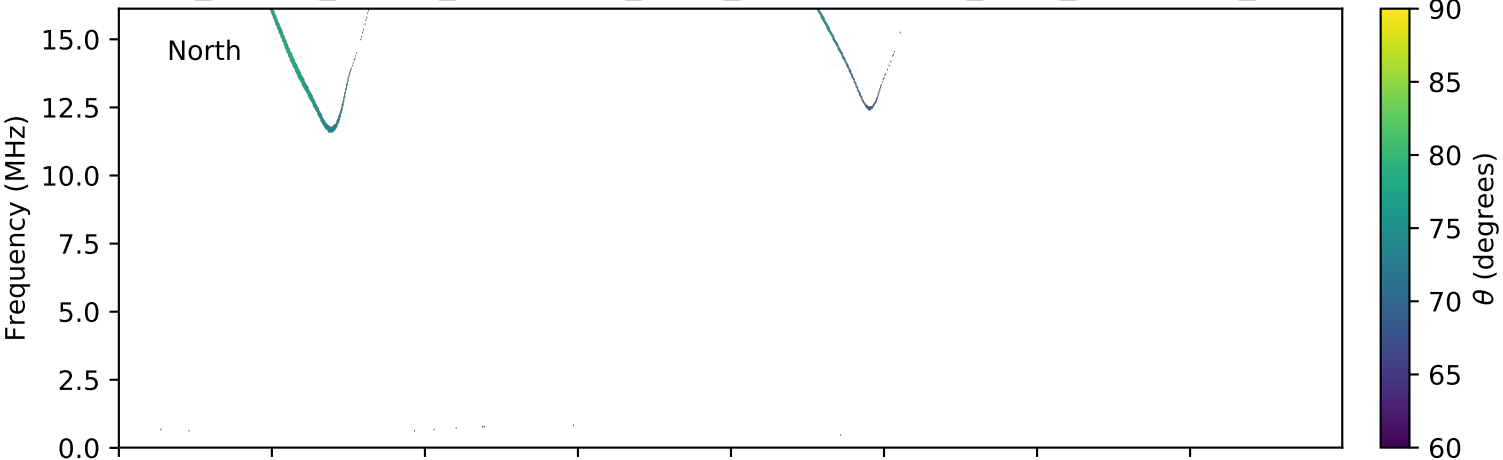
expres_cassini_jupiter_ganymede_isaac_lossc-wid1deg_3kev_20000501_v01.cdf
