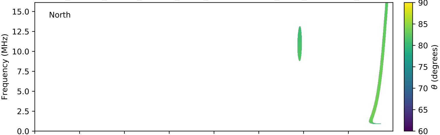
expres_cassini_jupiter_europa_isaac_lossc-wid1deg_3kev_20000528_v01.cdf
